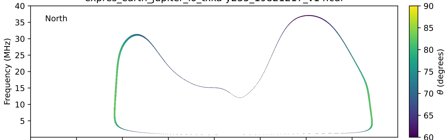
expres_earth_jupiter_io_txka-y235_19821217_v14.cdf
