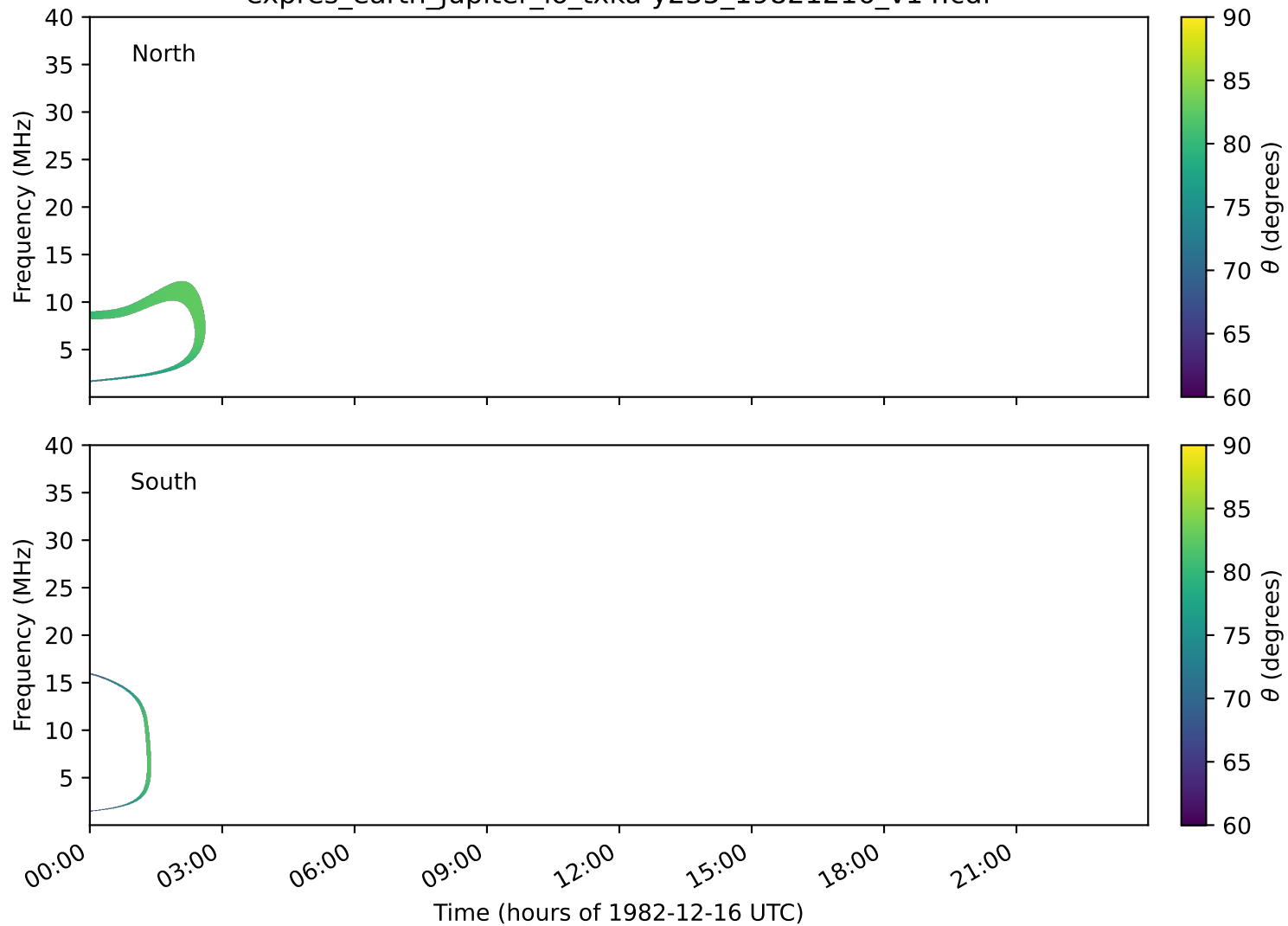
expres_earth_jupiter_io_txka-y235_19821216_v14.cdf
