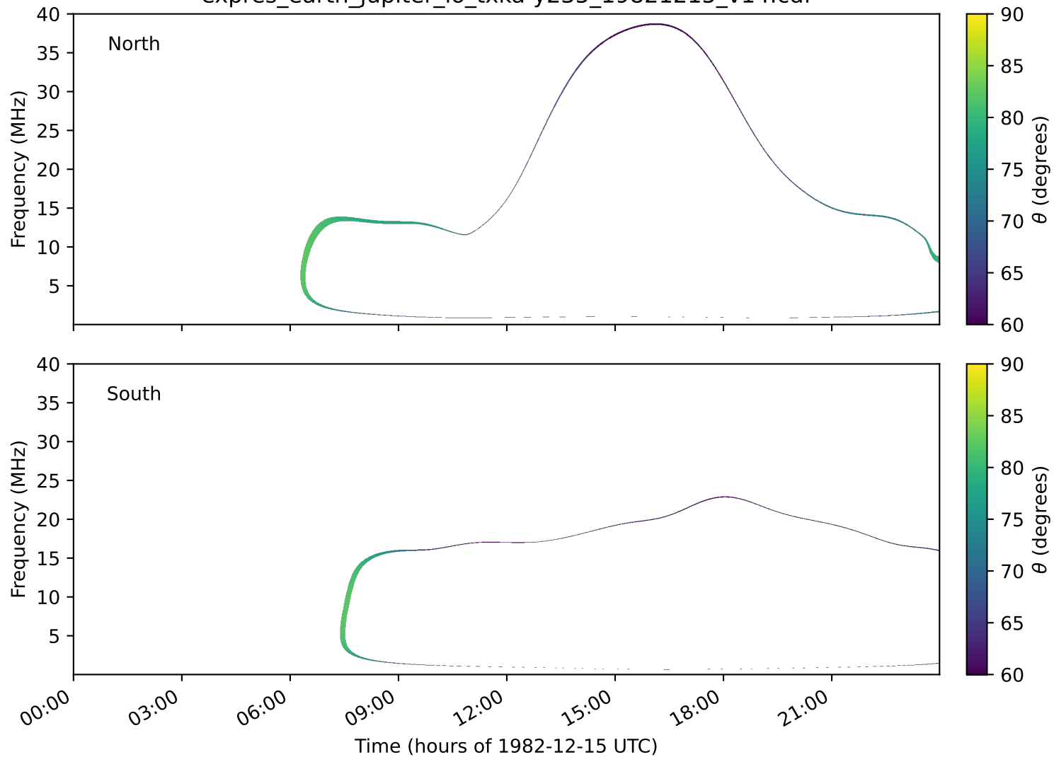
expres_earth_jupiter_io_txka-y235_19821215_v14.cdf
