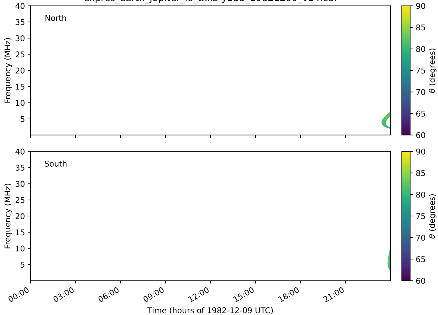
expres_earth_jupiter_io_txka-y235_19821209_v14.cdf
