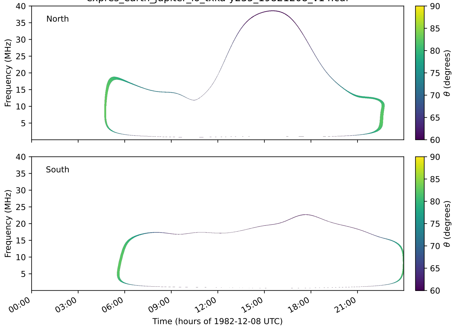
expres_earth_jupiter_io_txka-y235_19821208_v14.cdf
