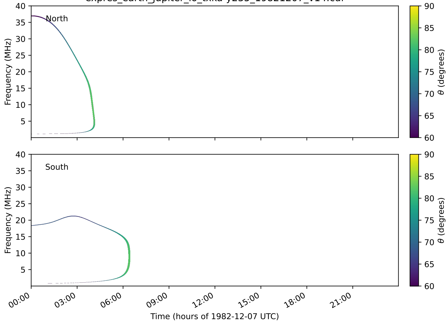
expres_earth_jupiter_io_txka-y235_19821207_v14.cdf
