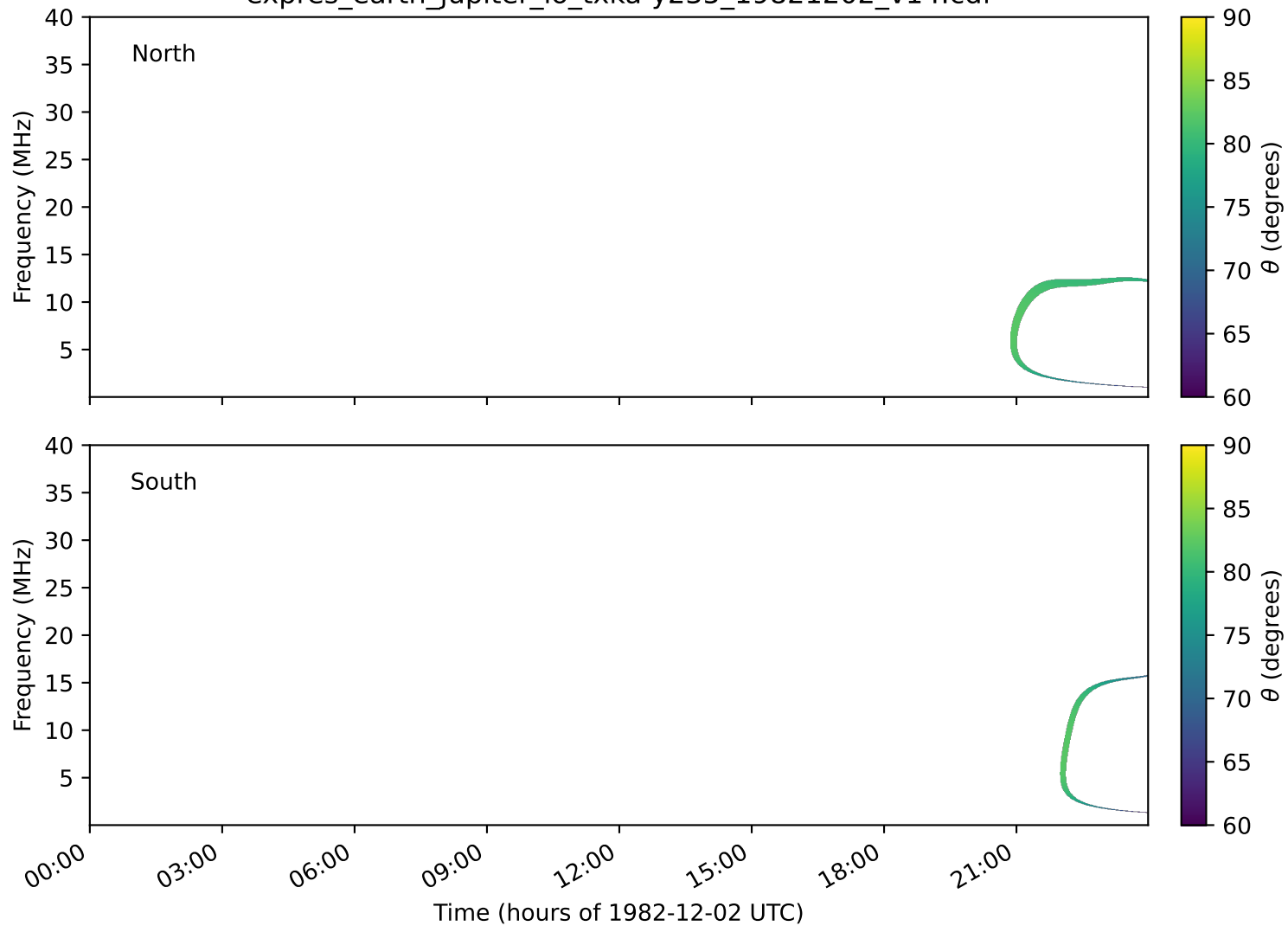
expres_earth_jupiter_io_txka-y235_19821202_v14.cdf
