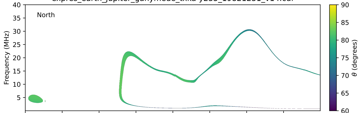
expres_earth_jupiter_ganymede_txka-y235_19821231_v14.cdf
