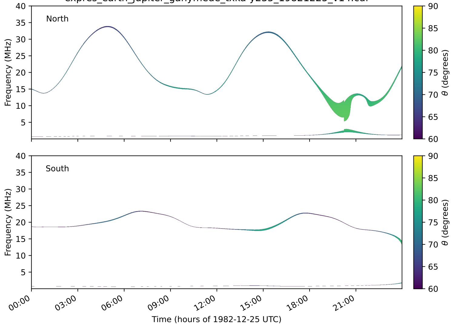
expres_earth_jupiter_ganymede_txka-y235_19821225_v14.cdf
