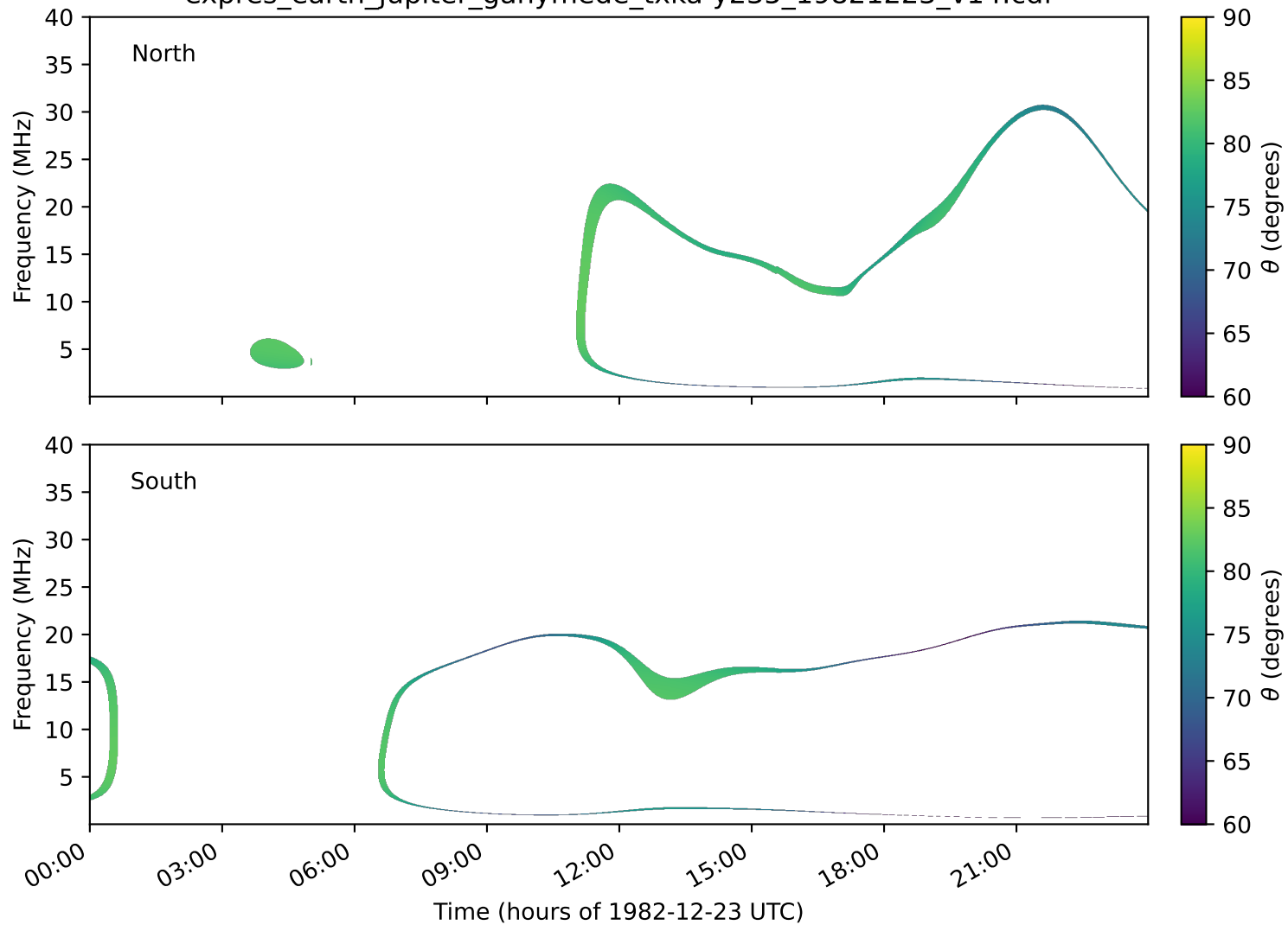
expres_earth_jupiter_ganymede_txka-y235_19821223_v14.cdf
