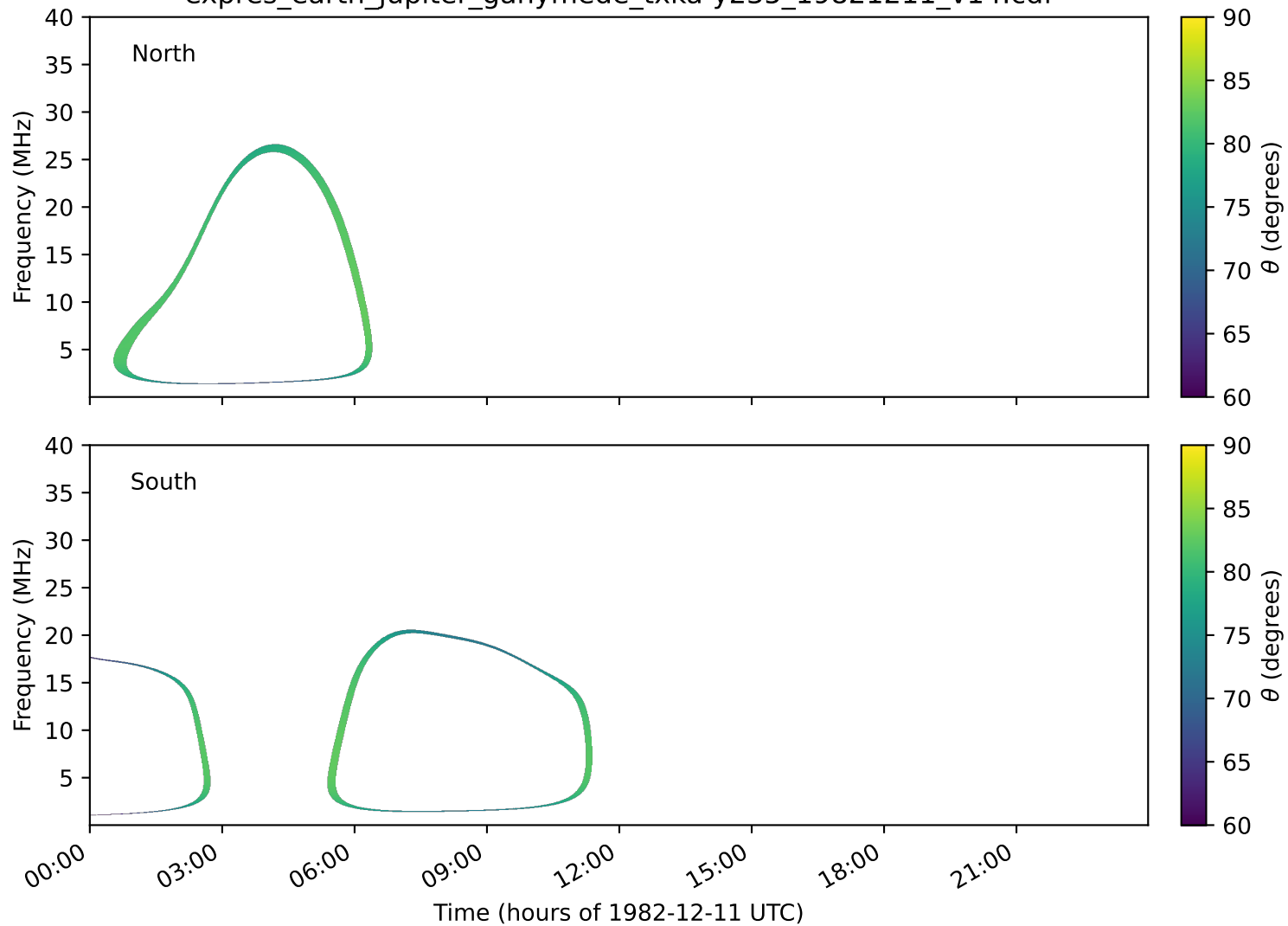
expres_earth_jupiter_ganymede_txka-y235_19821211_v14.cdf
