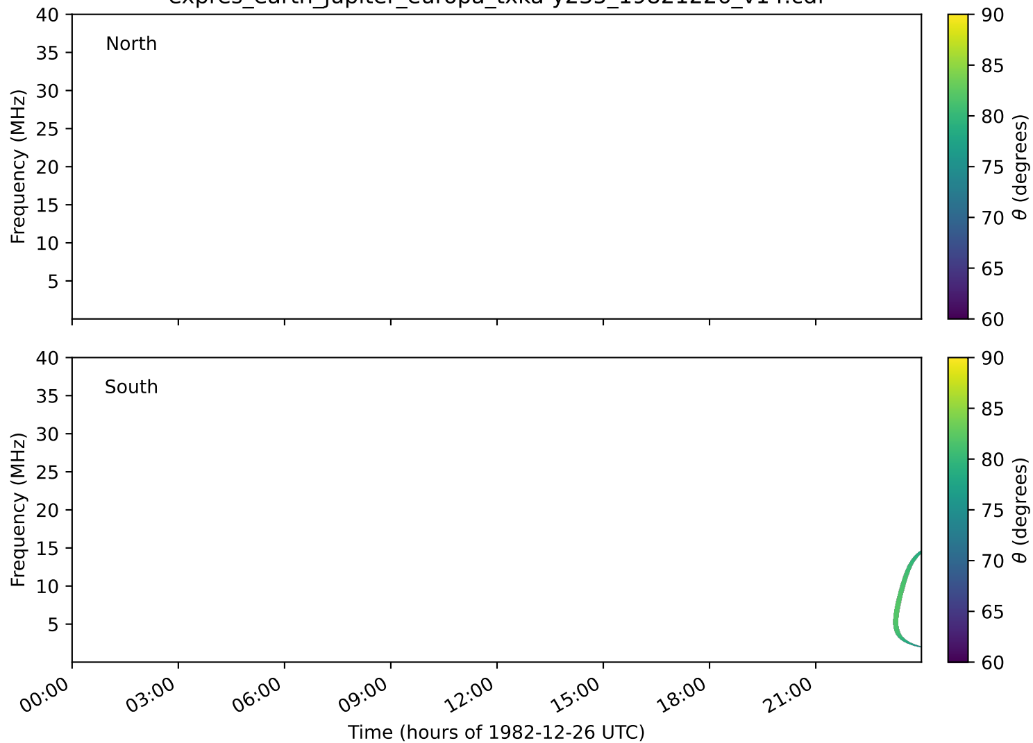
expres_earth_jupiter_europa_txka-y235_19821226_v14.cdf
