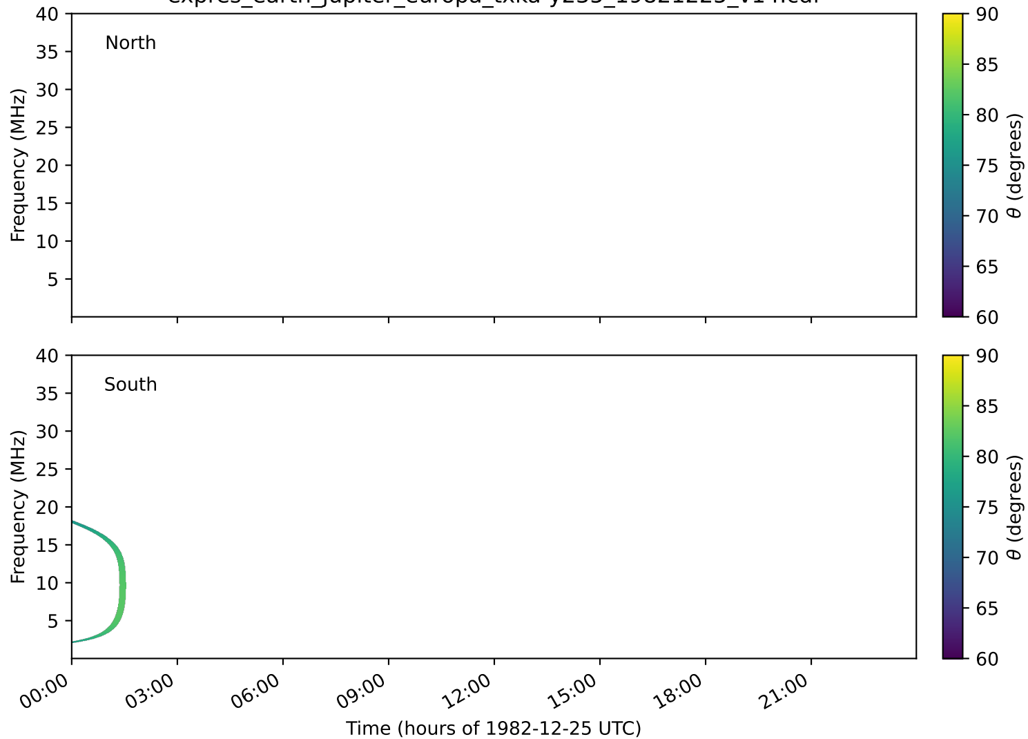
expres_earth_jupiter_europa_txka-y235_19821225_v14.cdf
