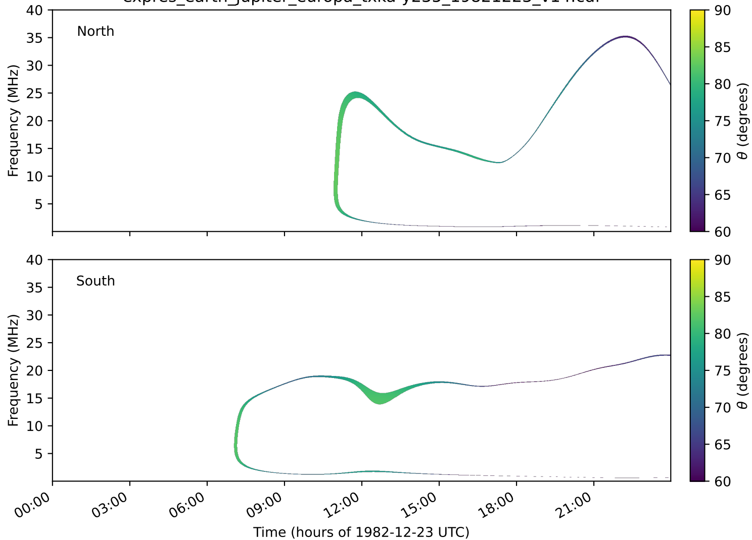
expres_earth_jupiter_europa_txka-y235_19821223_v14.cdf
