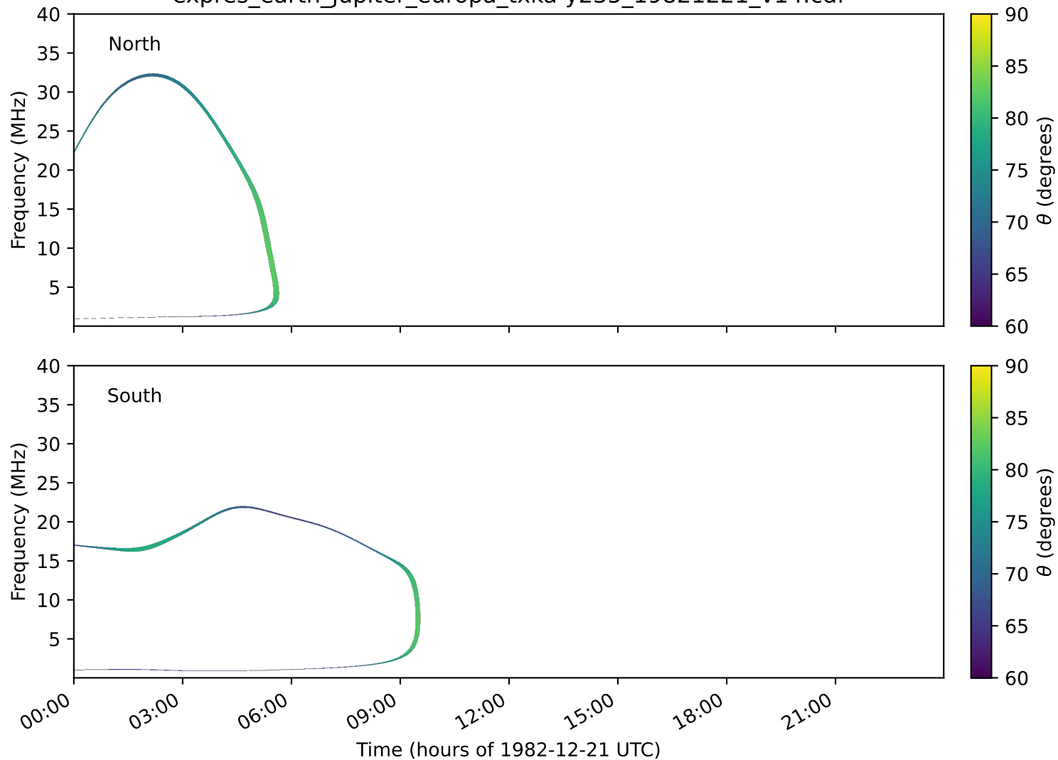
expres_earth_jupiter_europa_txka-y235_19821221_v14.cdf
