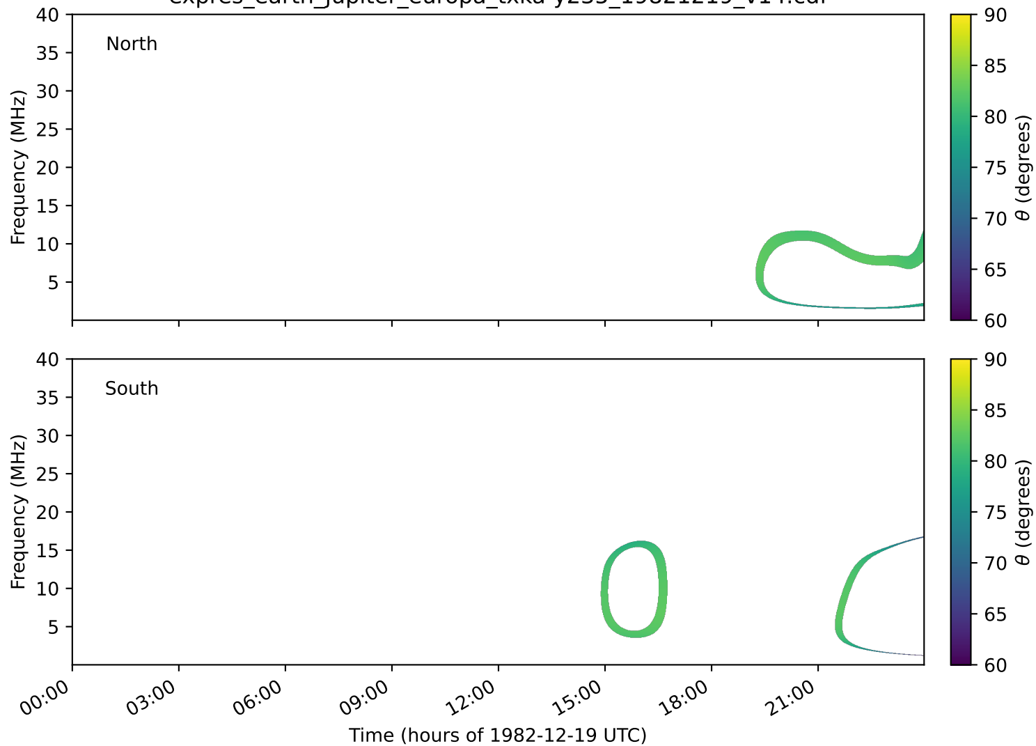
expres_earth_jupiter_europa_txka-y235_19821219_v14.cdf
