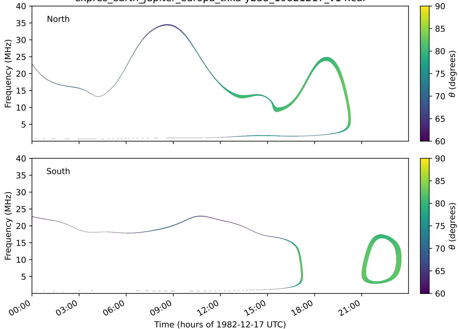
expres_earth_jupiter_europa_txka-y235_19821217_v14.cdf
