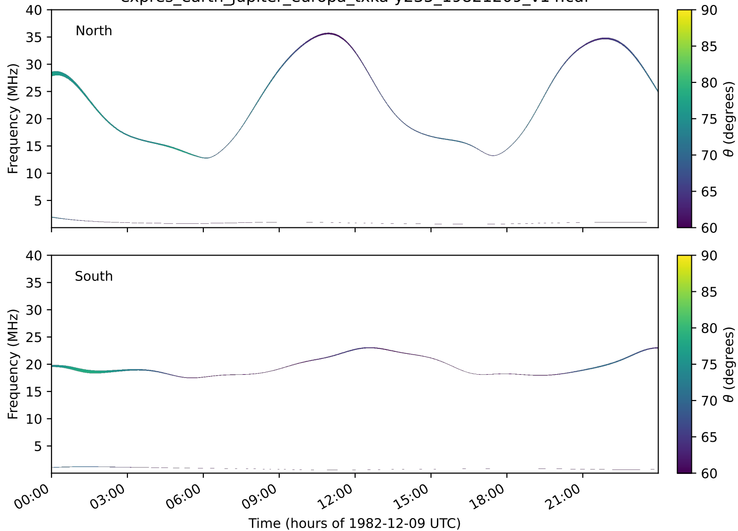
expres_earth_jupiter_europa_txka-y235_19821209_v14.cdf
