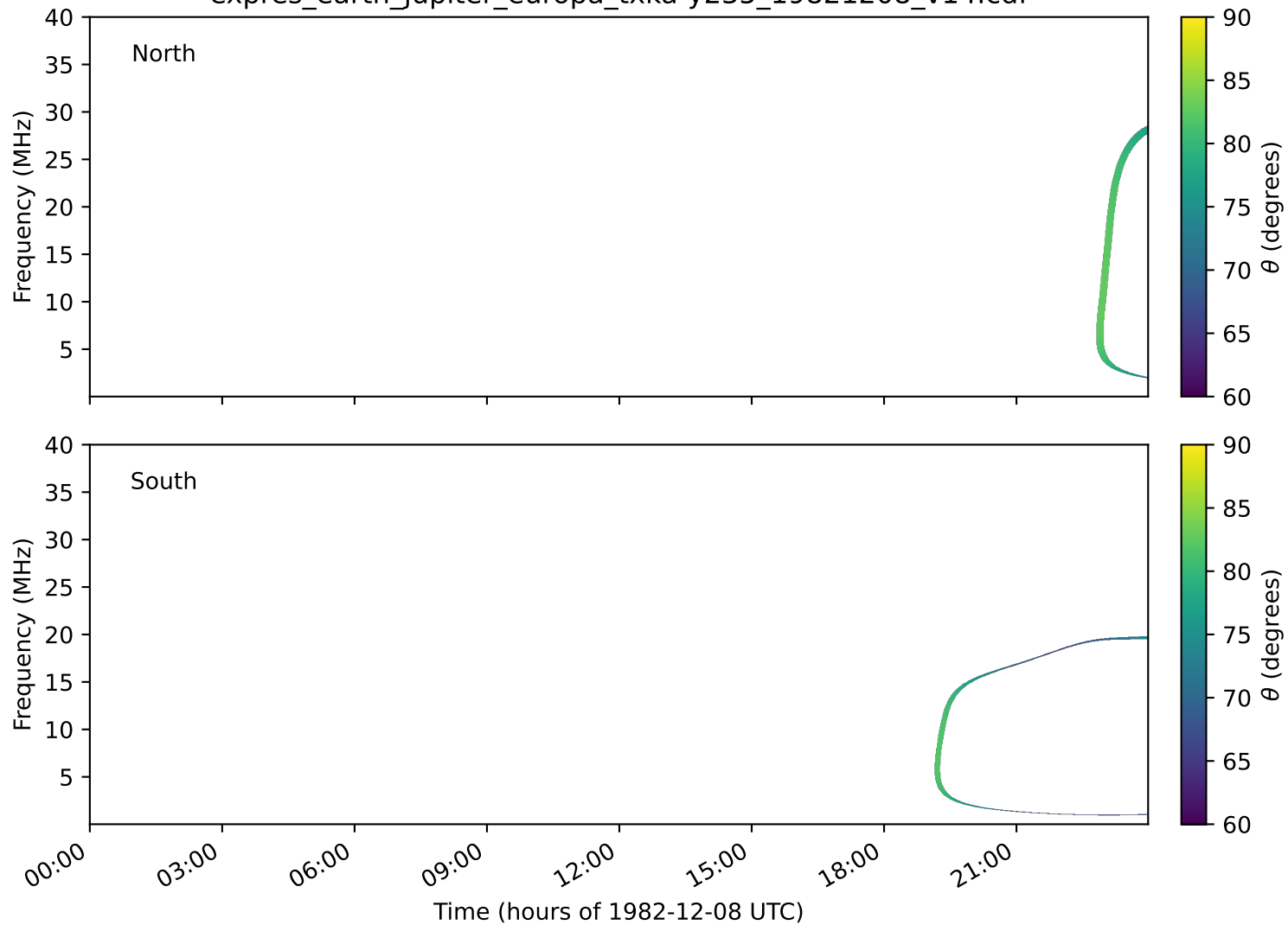
expres_earth_jupiter_europa_txka-y235_19821208_v14.cdf
