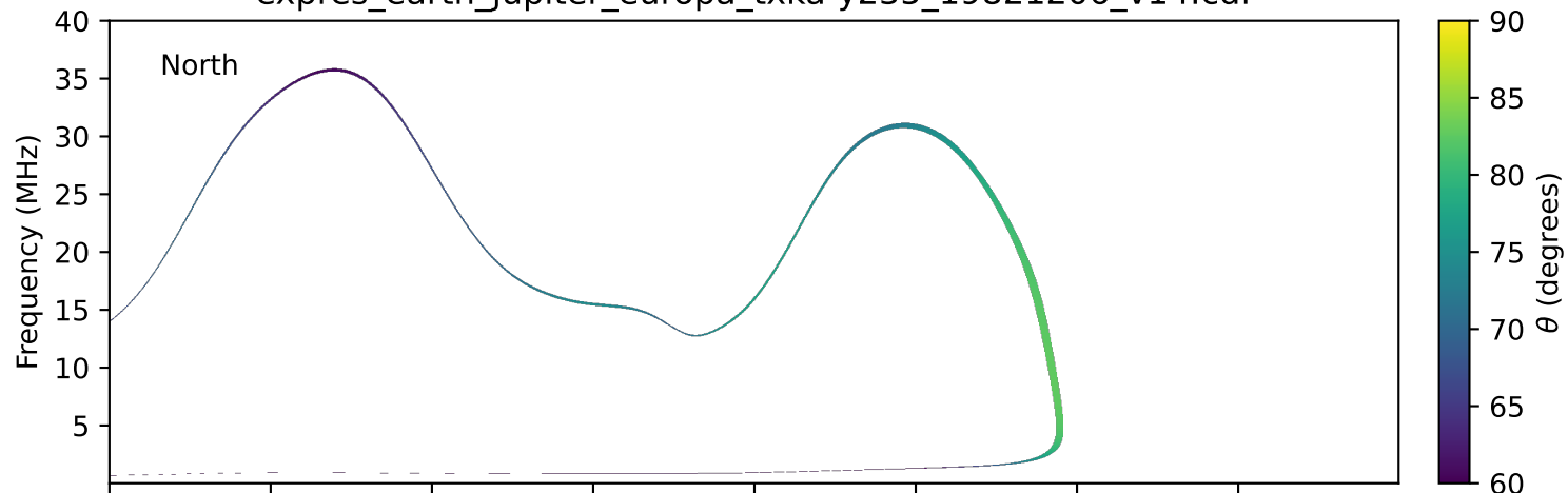
expres_earth_jupiter_europa_txka-y235_19821206_v14.cdf
