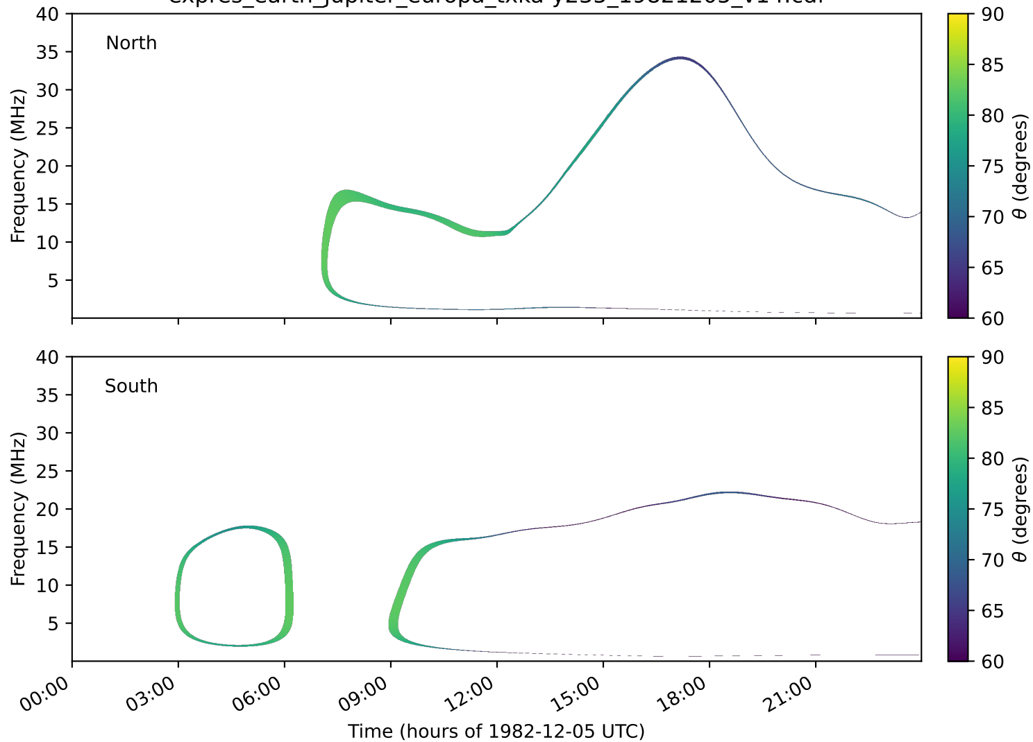
expres_earth_jupiter_europa_txka-y235_19821205_v14.cdf
