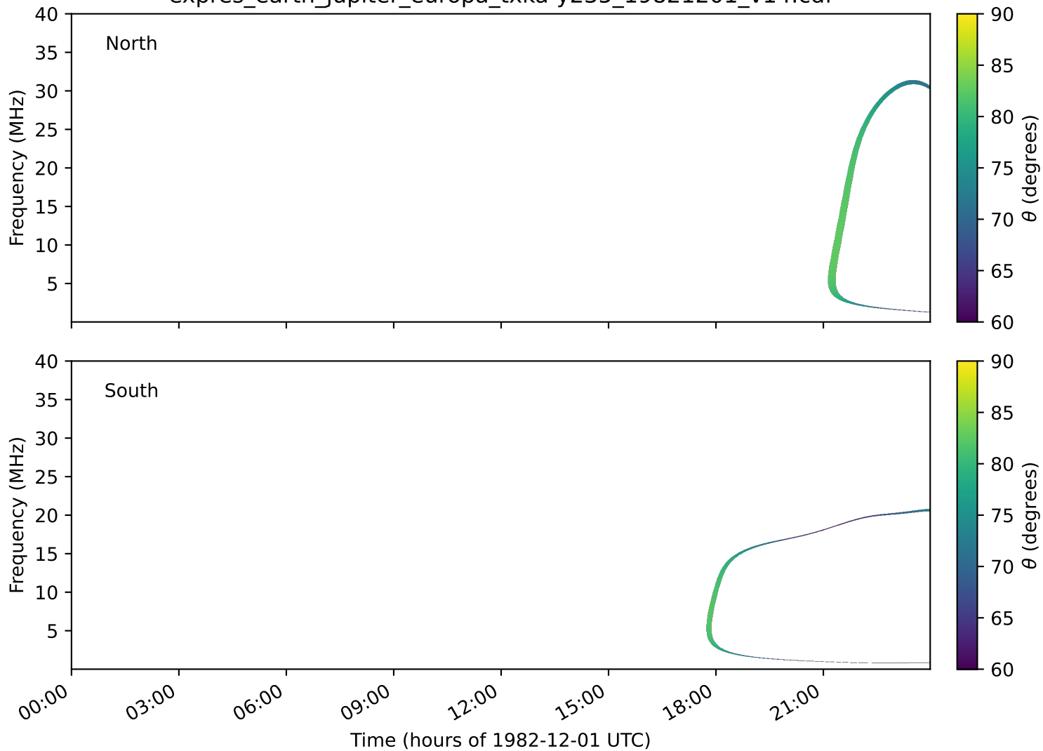
expres_earth_jupiter_europa_txka-y235_19821201_v14.cdf
