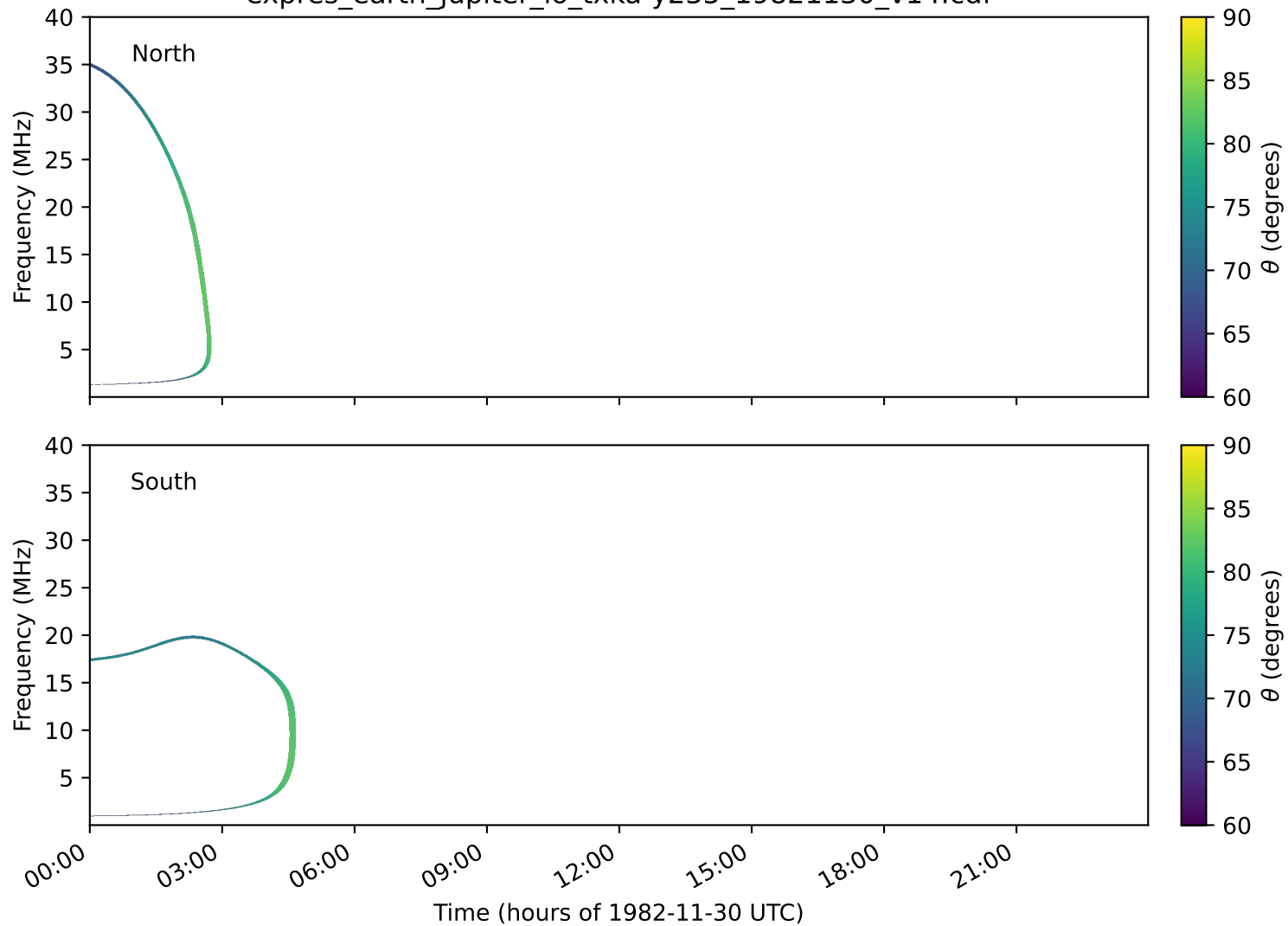
expres_earth_jupiter_io_txka-y235_19821130_v14.cdf
