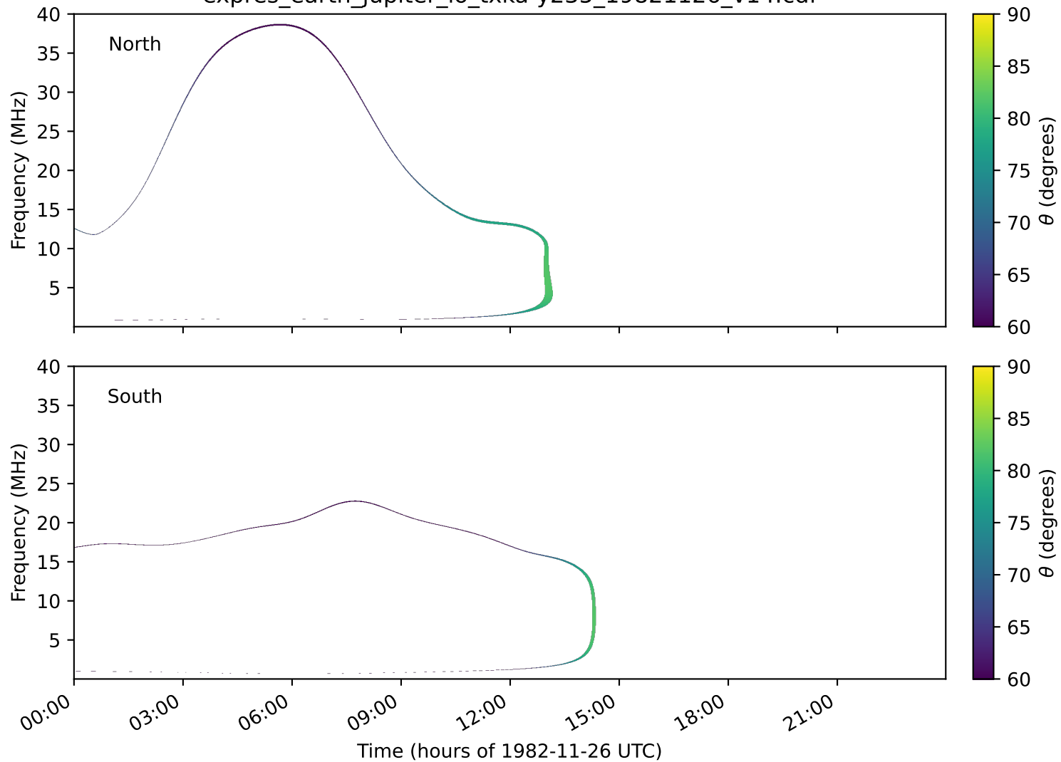
expres_earth_jupiter_io_txka-y235_19821126_v14.cdf
