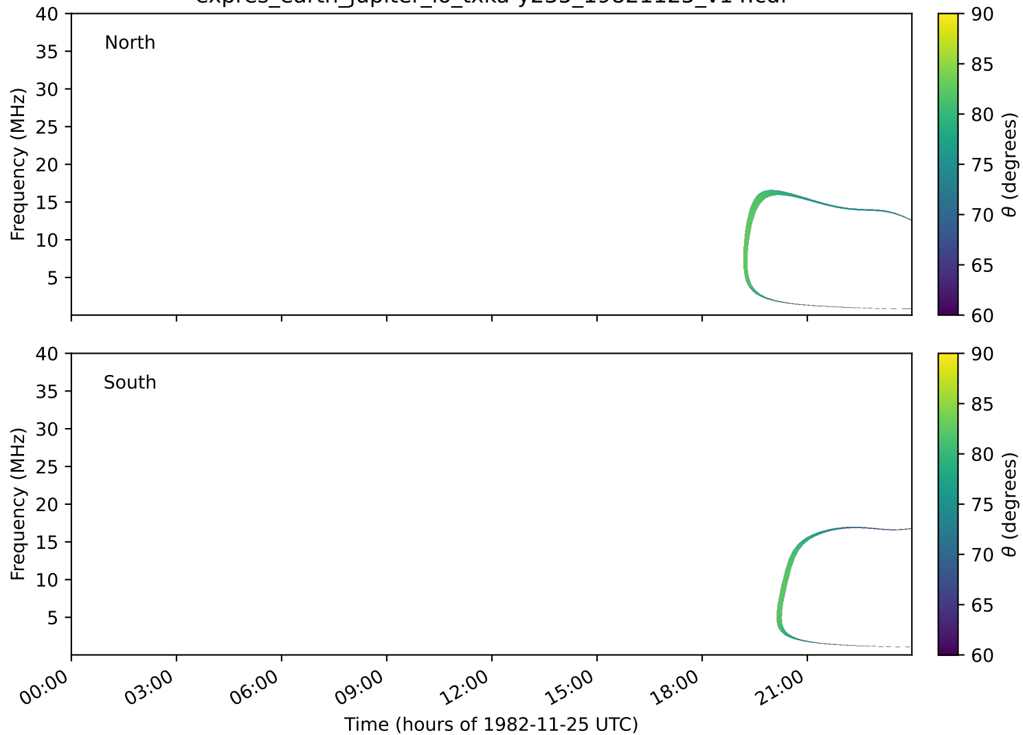
expres_earth_jupiter_io_txka-y235_19821125_v14.cdf
