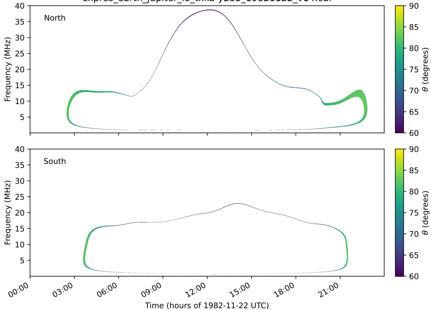
expres_earth_jupiter_io_txka-y235_19821122_v14.cdf
