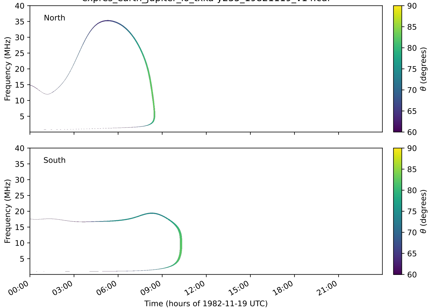
expres_earth_jupiter_io_txka-y235_19821119_v14.cdf
