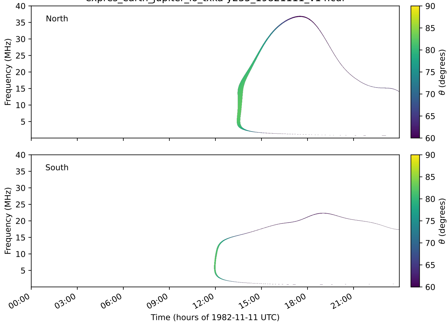
expres_earth_jupiter_io_txka-y235_19821111_v14.cdf
