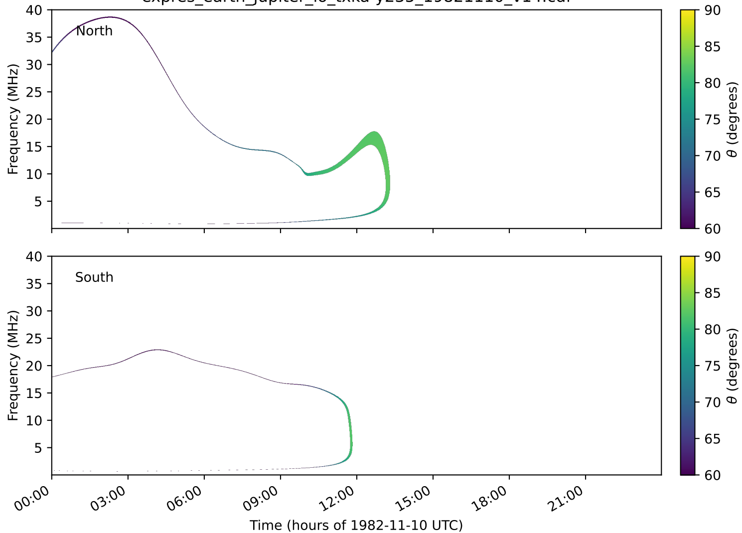
expres_earth_jupiter_io_txka-y235_19821110_v14.cdf
