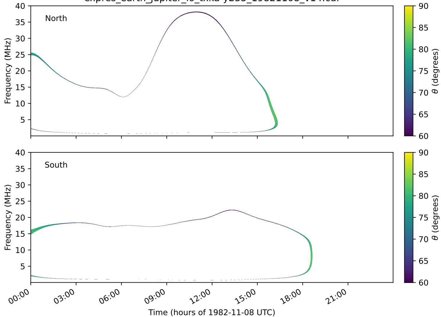
expres_earth_jupiter_io_txka-y235_19821108_v14.cdf
