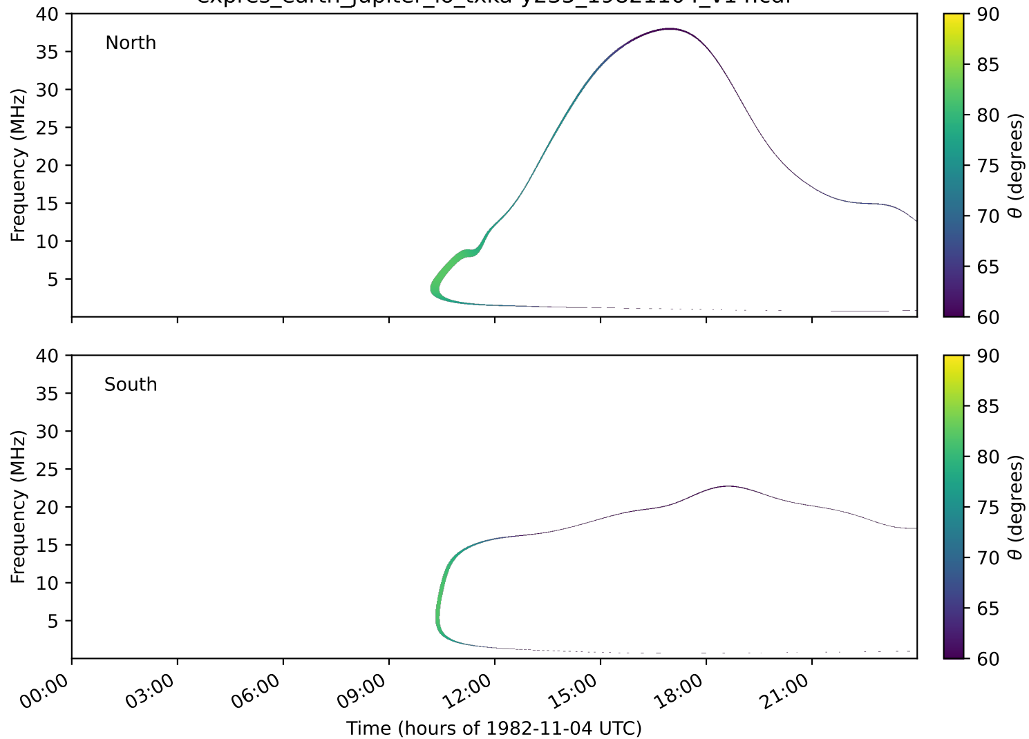
expres_earth_jupiter_io_txka-y235_19821104_v14.cdf
