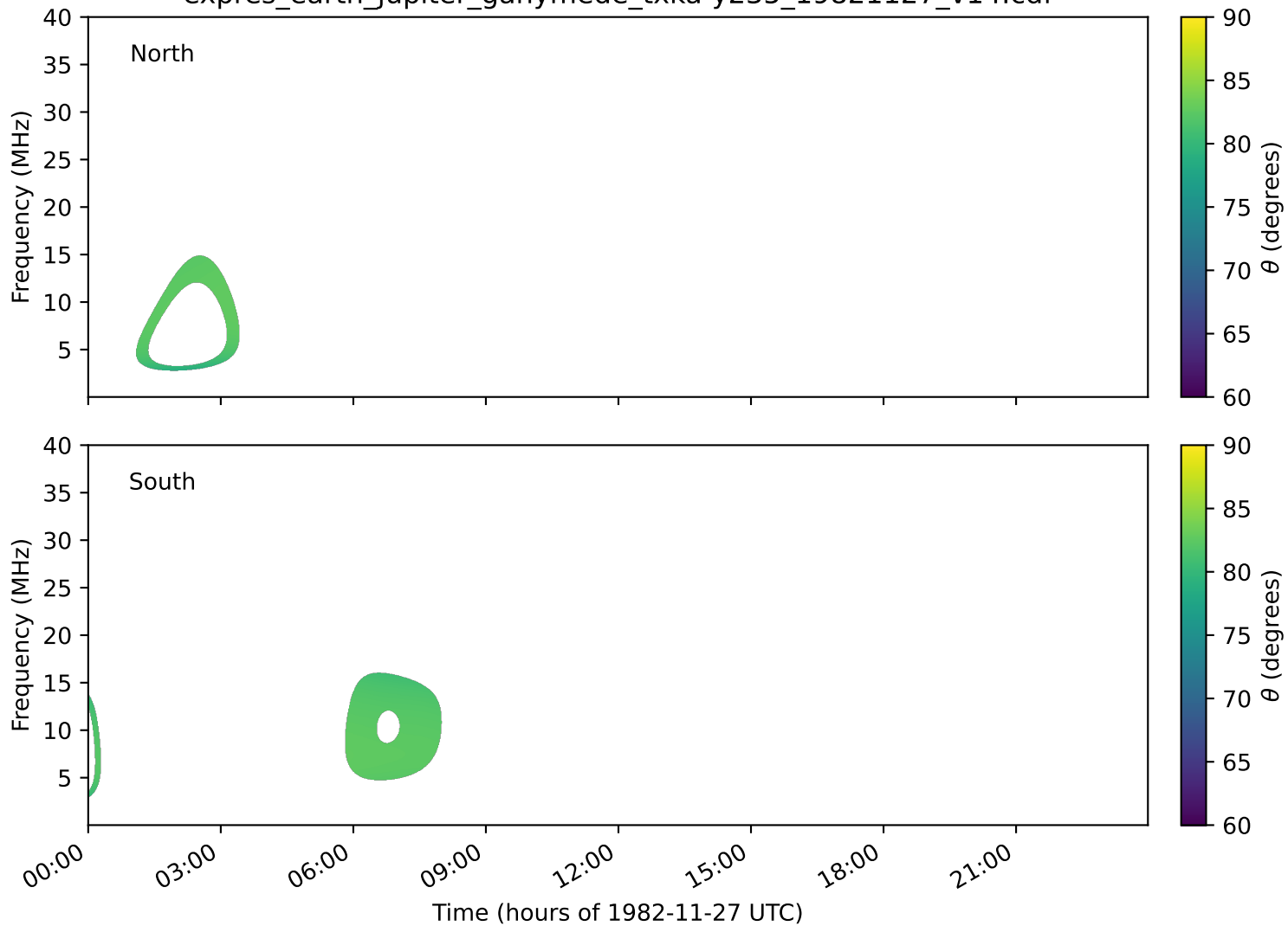
expres_earth_jupiter_ganymede_txka-y235_19821127_v14.cdf
