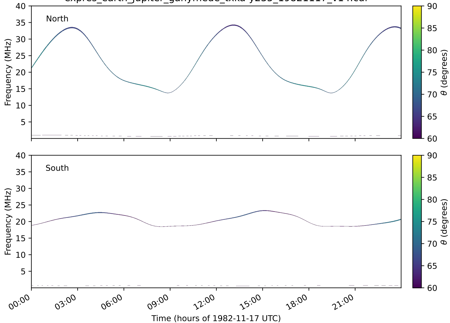
expres_earth_jupiter_ganymede_txka-y235_19821117_v14.cdf
