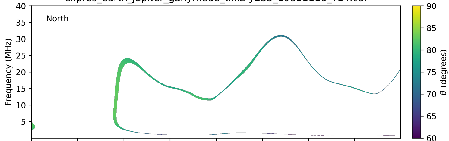
expres_earth_jupiter_ganymede_txka-y235_19821116_v14.cdf
