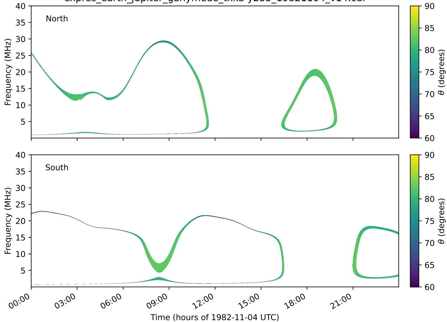
expres_earth_jupiter_ganymede_txka-y235_19821104_v14.cdf
