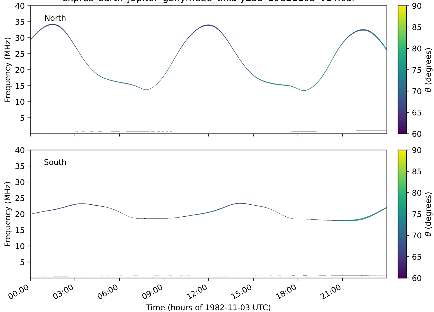
expres_earth_jupiter_ganymede_txka-y235_19821103_v14.cdf
