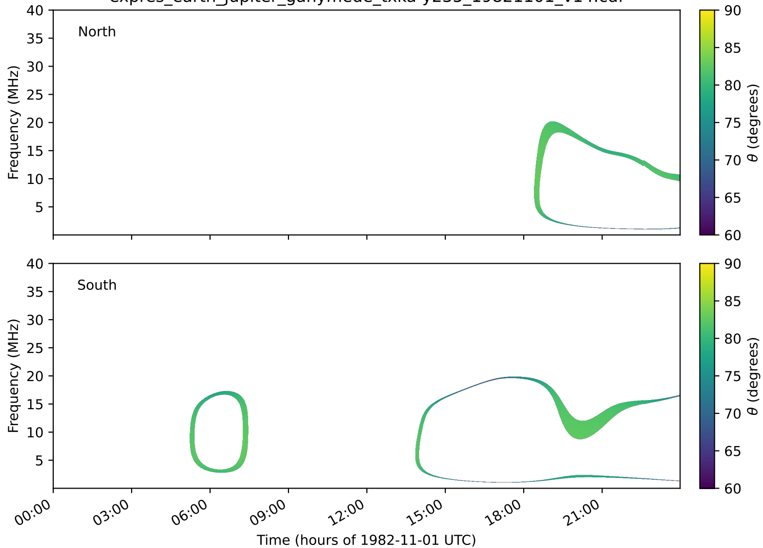
expres_earth_jupiter_ganymede_txka-y235_19821101_v14.cdf
