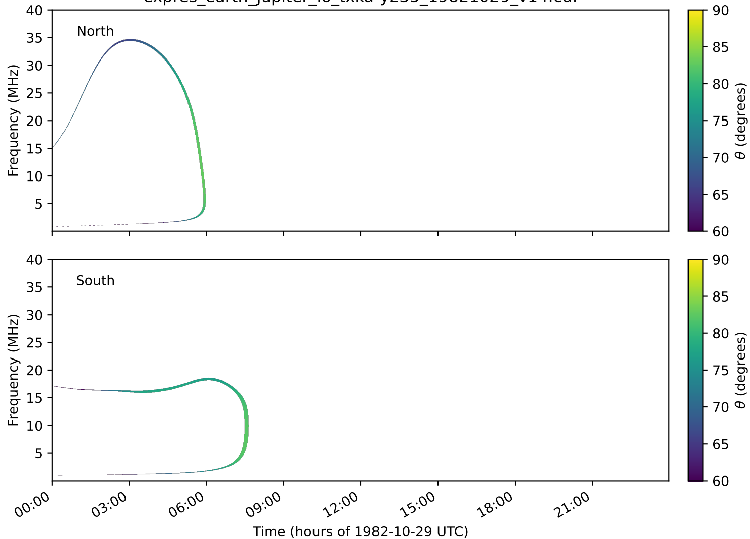
expres_earth_jupiter_io_txka-y235_19821029_v14.cdf
