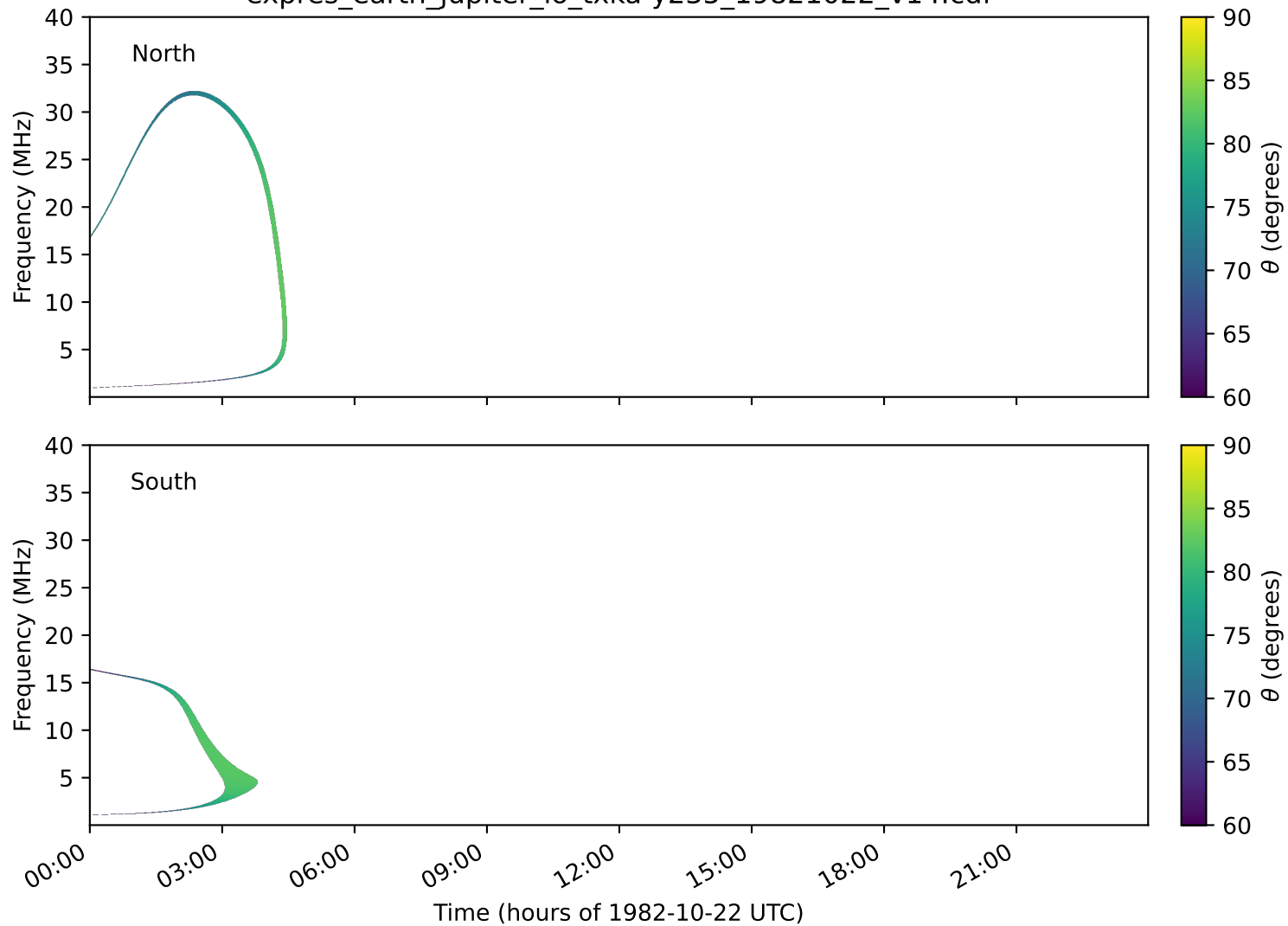
expres_earth_jupiter_io_txka-y235_19821022_v14.cdf
