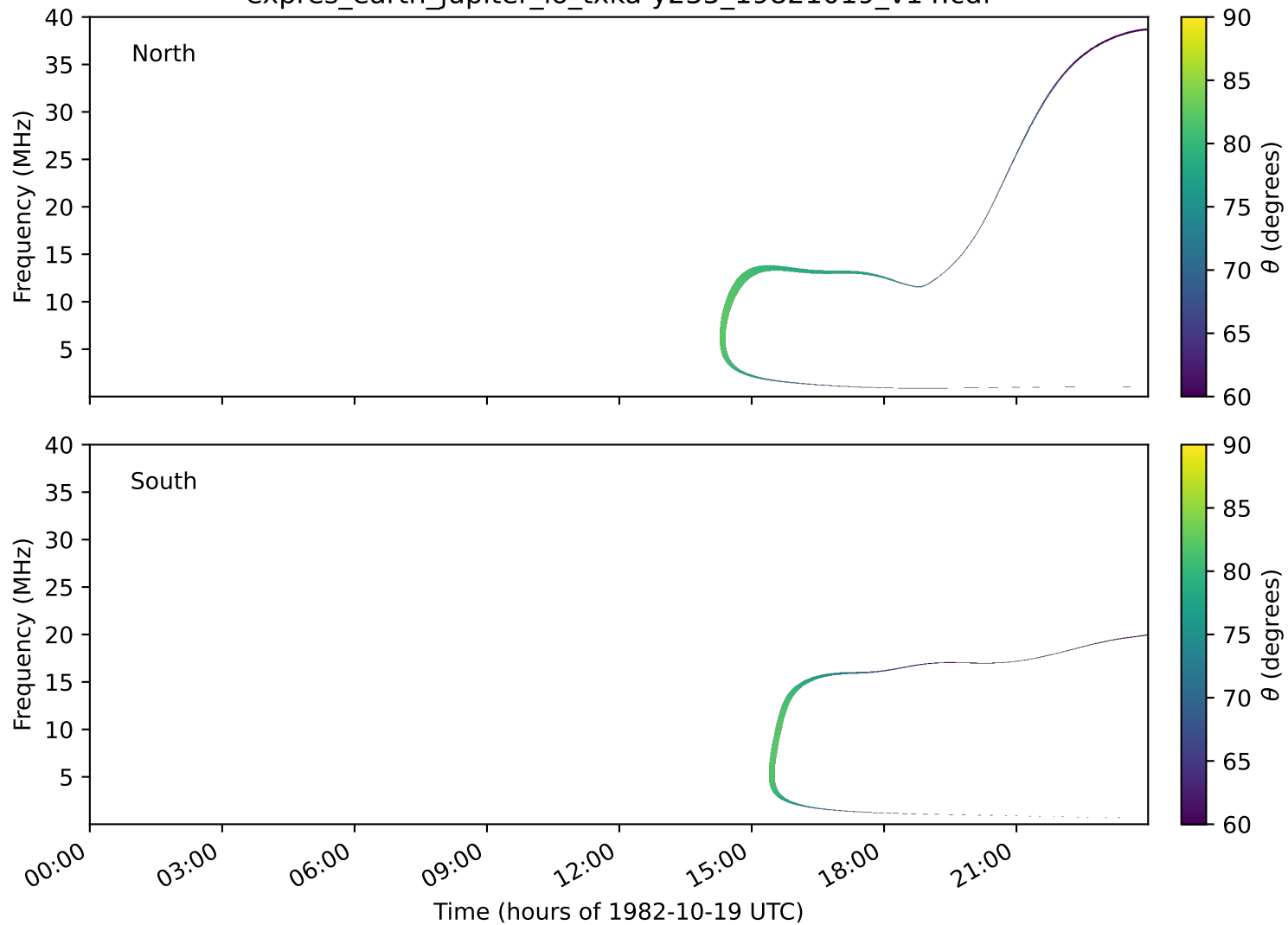
expres_earth_jupiter_io_txka-y235_19821019_v14.cdf
