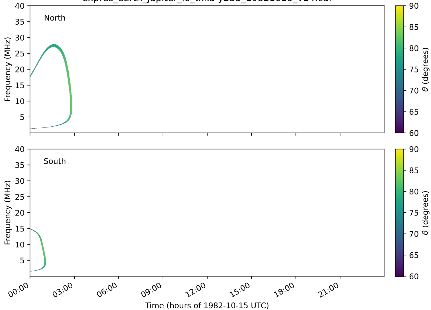
expres_earth_jupiter_io_txka-y235_19821015_v14.cdf
