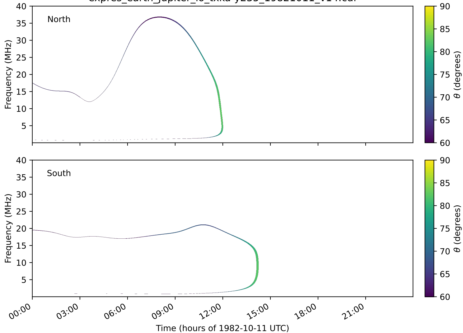
expres_earth_jupiter_io_txka-y235_19821011_v14.cdf
