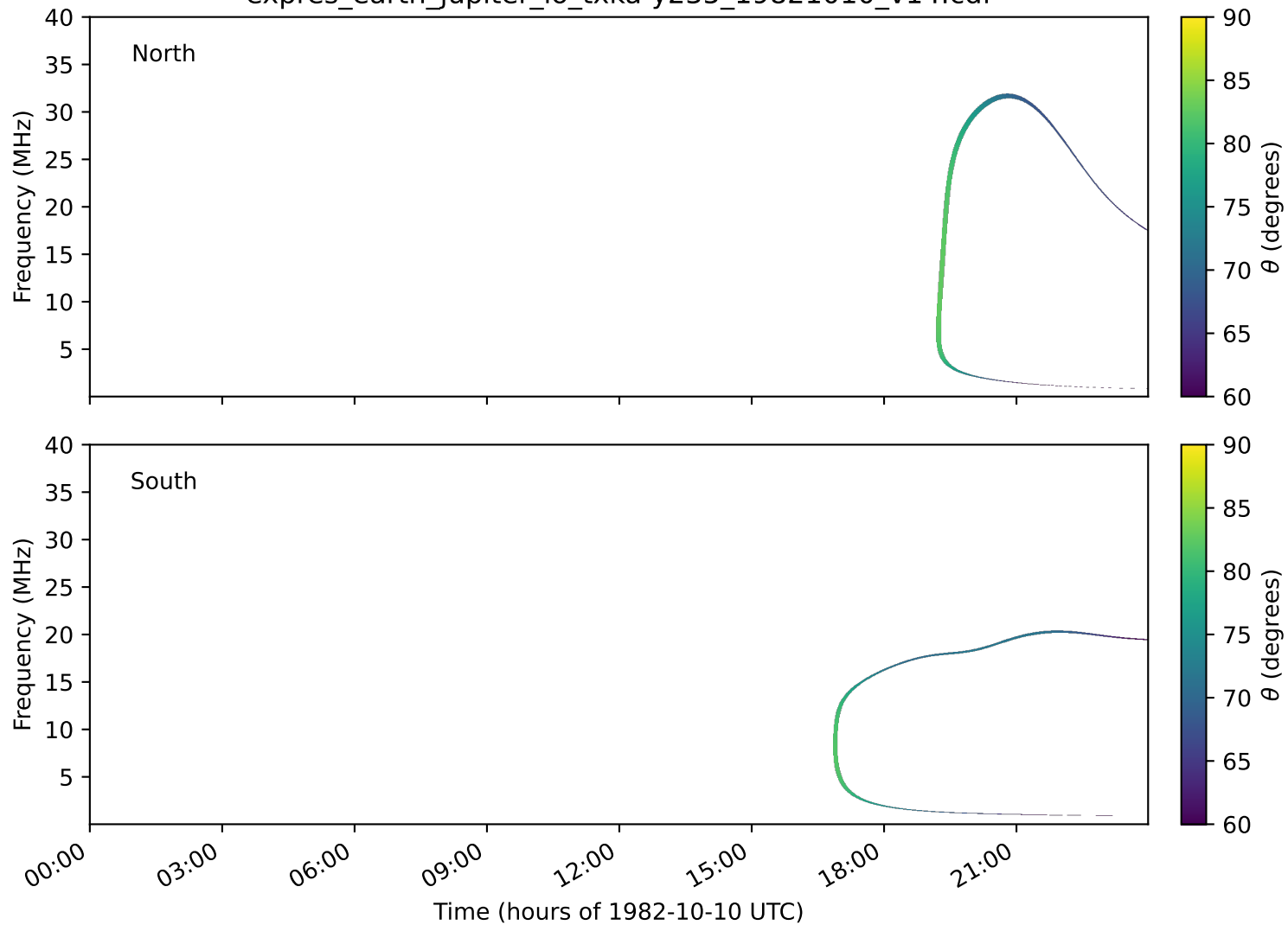
expres_earth_jupiter_io_txka-y235_19821010_v14.cdf
