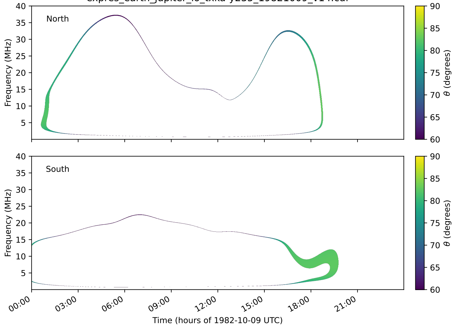
expres_earth_jupiter_io_txka-y235_19821009_v14.cdf
