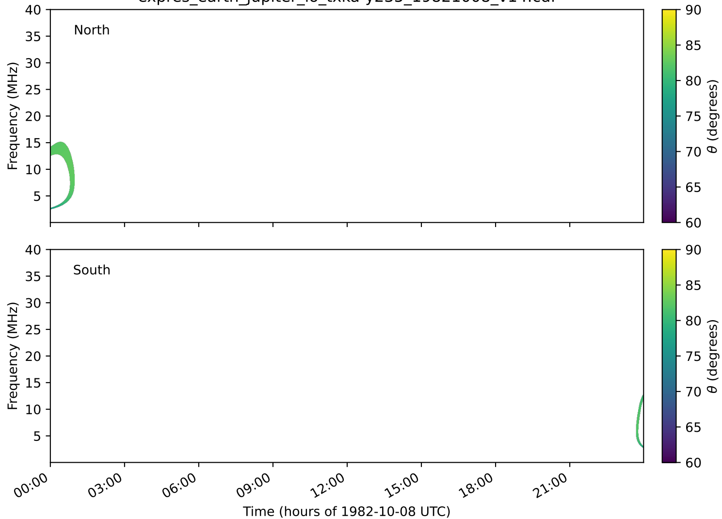
expres_earth_jupiter_io_txka-y235_19821008_v14.cdf
