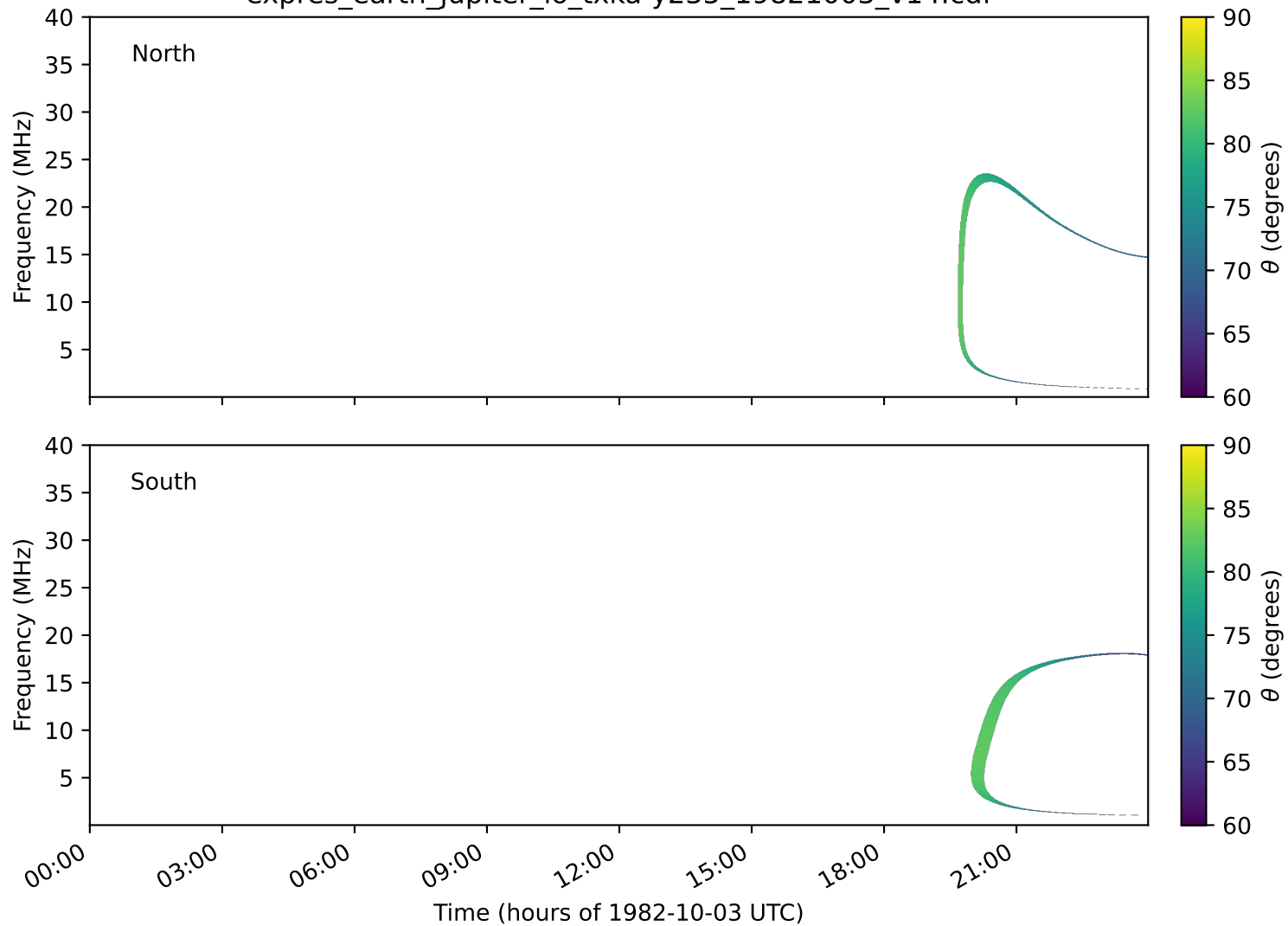
expres_earth_jupiter_io_txka-y235_19821003_v14.cdf
