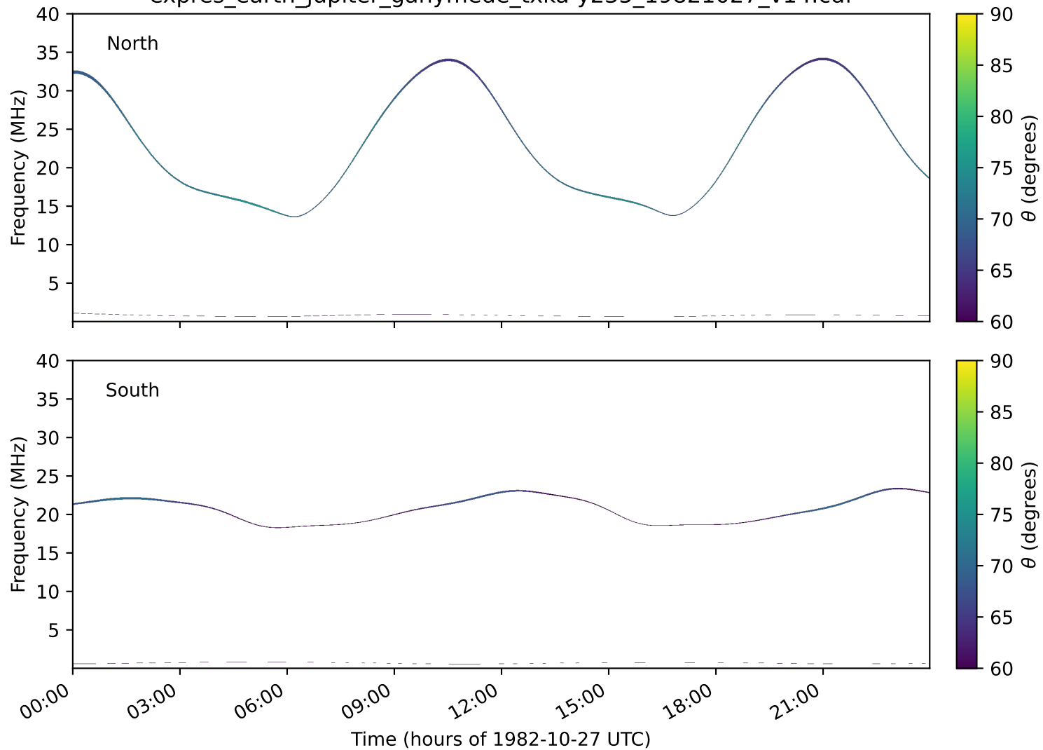
expres_earth_jupiter_ganymede_txka-y235_19821027_v14.cdf
