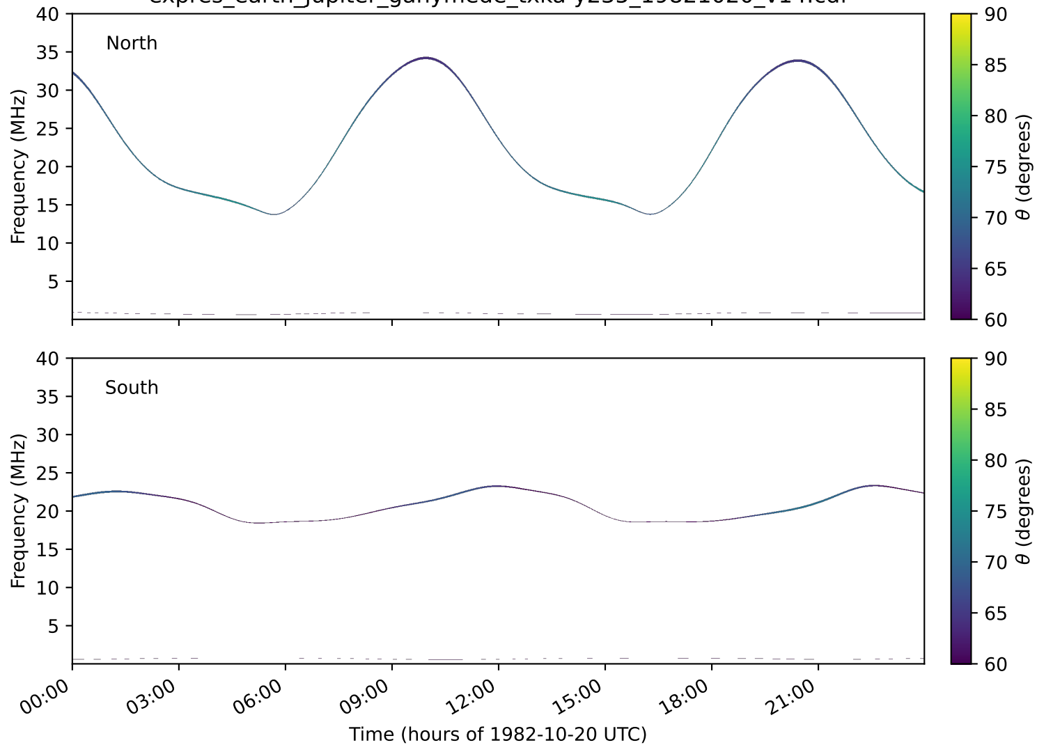
expres_earth_jupiter_ganymede_txka-y235_19821020_v14.cdf
