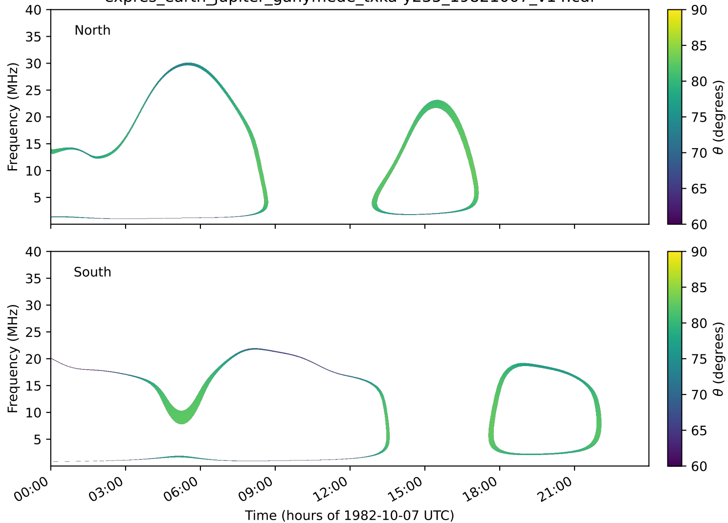
expres_earth_jupiter_ganymede_txka-y235_19821007_v14.cdf
