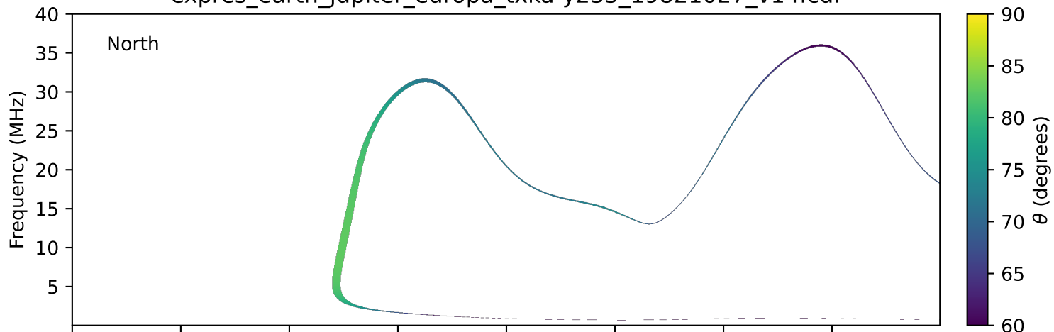
expres_earth_jupiter_europa_txka-y235_19821027_v14.cdf
